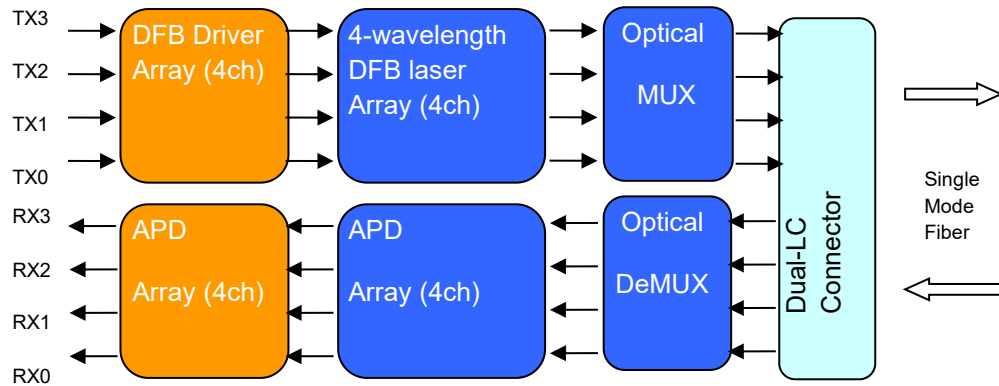
40Gb/s QSFP ZR4 Transceiver Block Diagram
