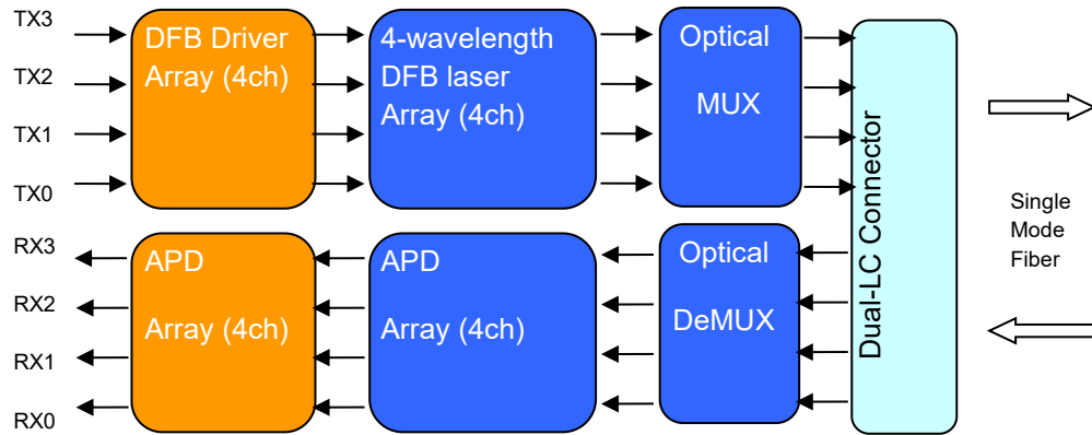
40Gb/s QSFP ZR4-Lite Transceiver Block Diagram
