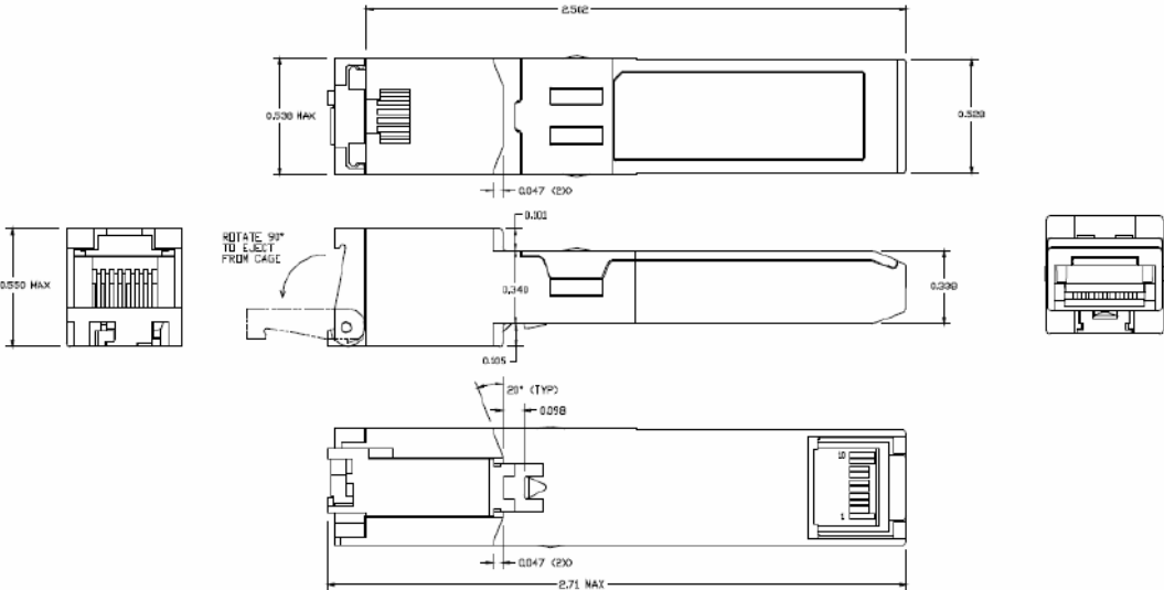
Figure 2. AOT-P-F(S) mechanical dimensions
