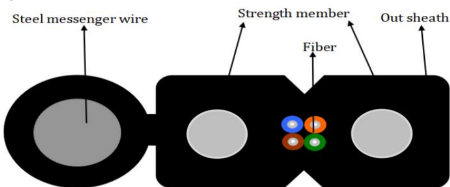
<Cross-sectional Drawing of Cable>
