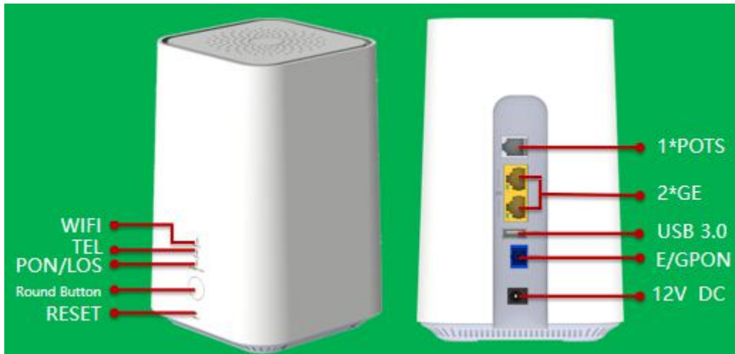
Figure 1 2GE+1POTS+1USB+WiFi4/5 HGU
